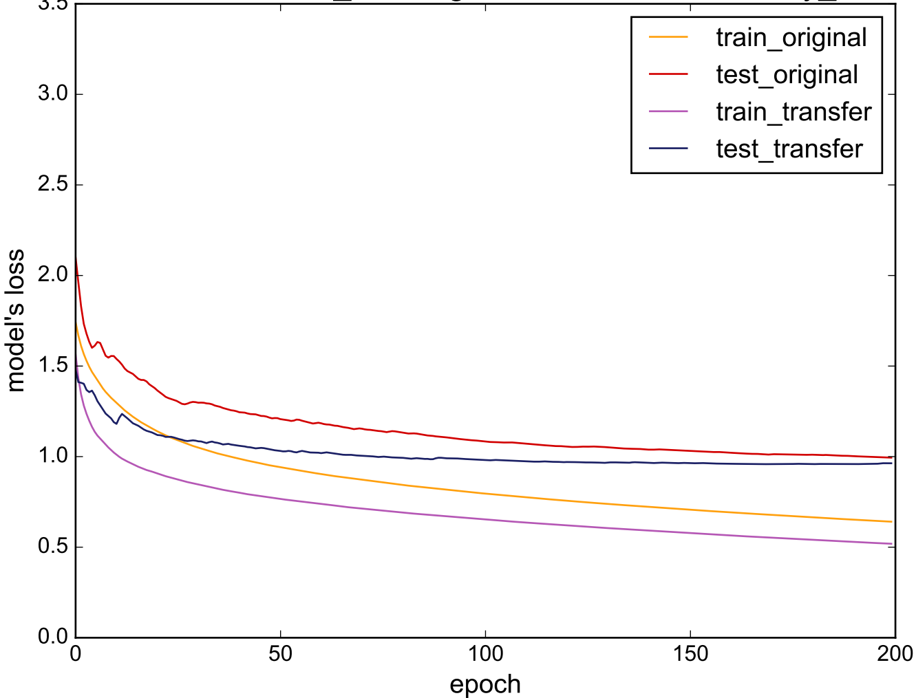
Source: Cricket_Y - Target: uWaveGestureLibrary_Z
