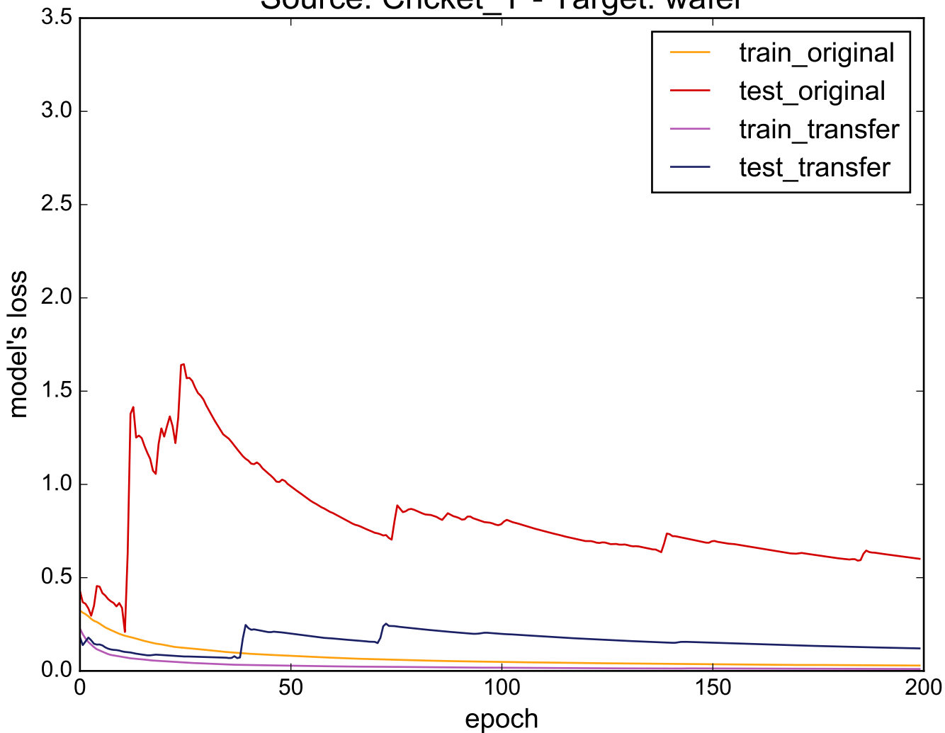
Source: Cricket_Y - Target: wafer
