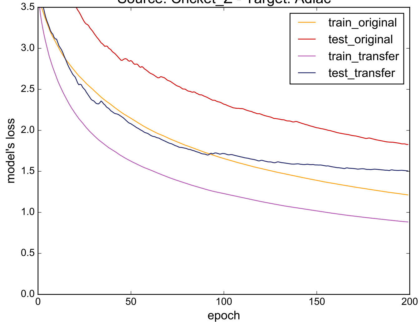
Source: Cricket_Z - Target: Adiac
