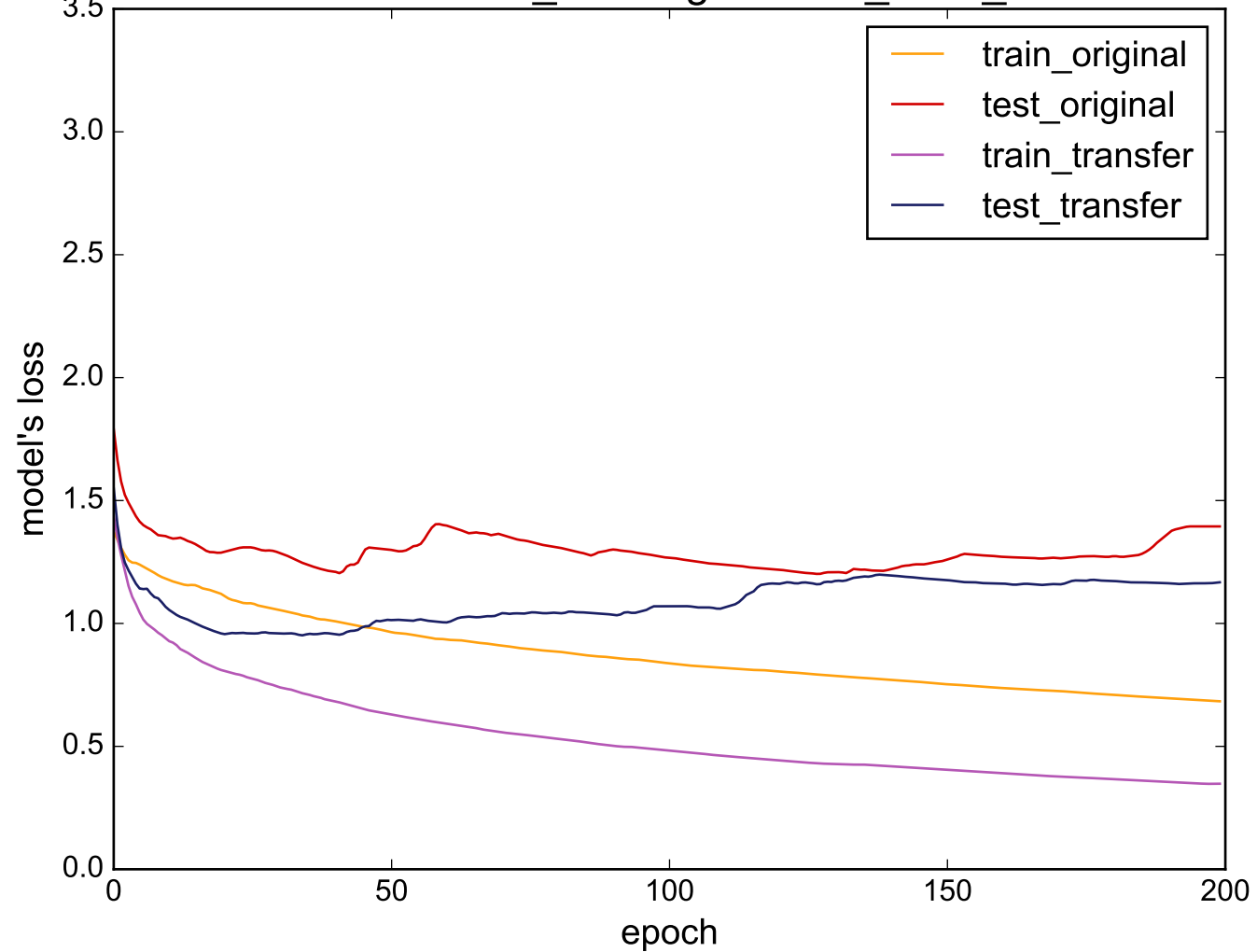
Source: Cricket_Z - Target: CinC_ECG_torso
