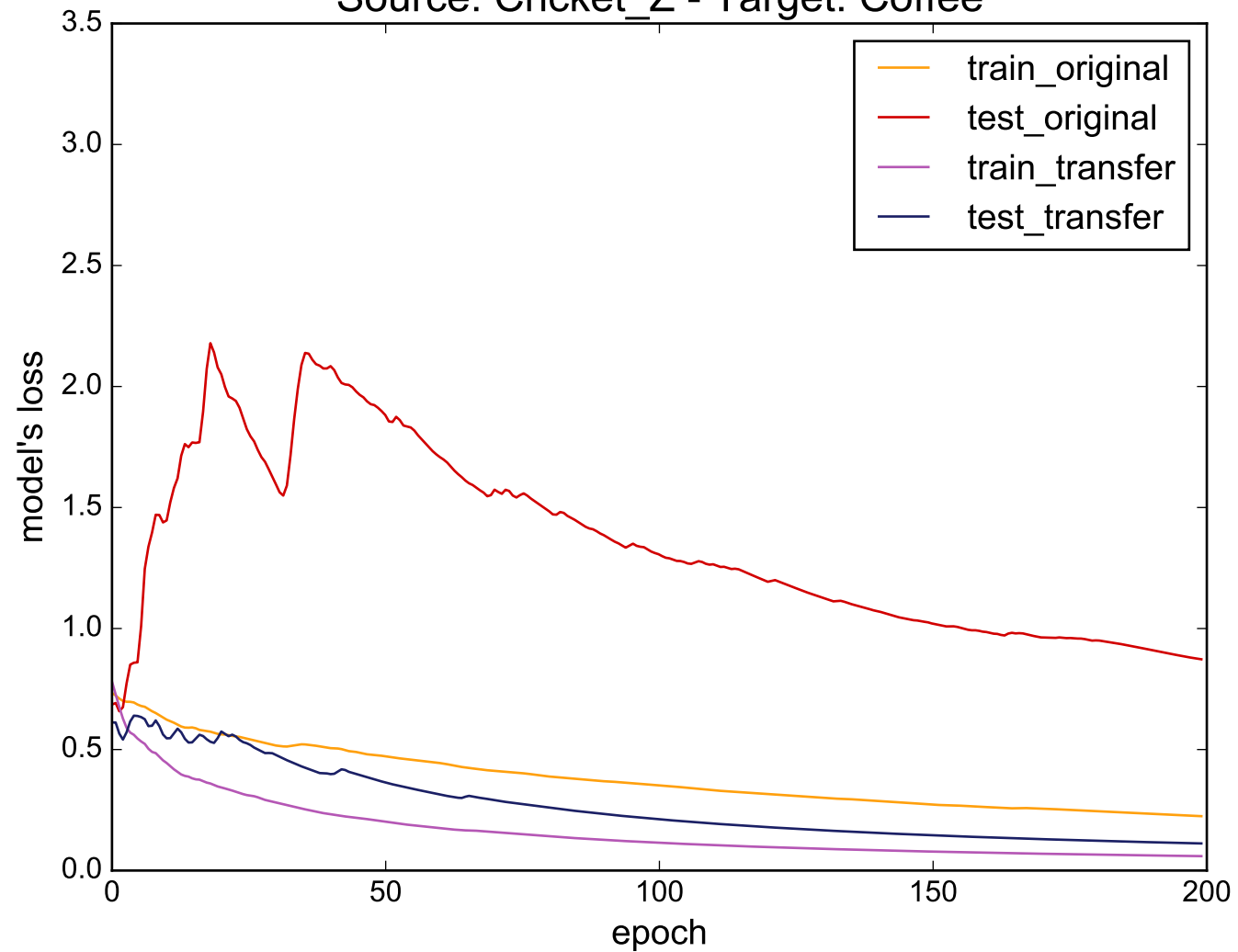
Source: Cricket_Z - Target: Coffee
