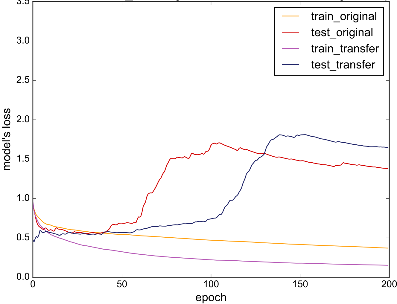
Source: Cricket_Z - Target: DistalPhalanxOutlineAgeGroup
