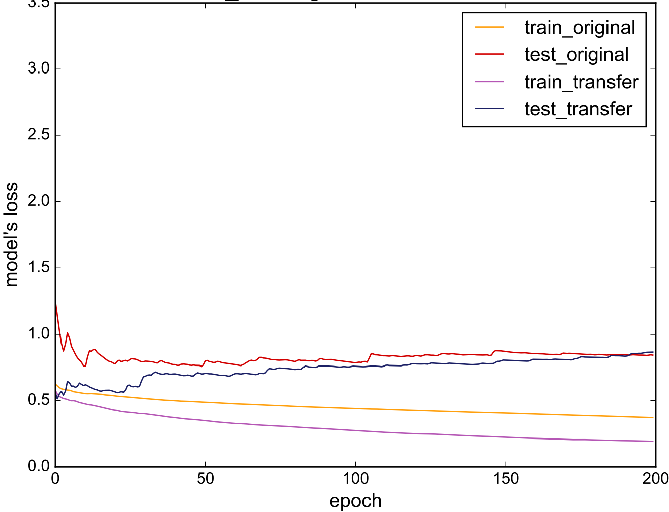
Source: Cricket_Z - Target: DistalPhalanxOutlineCorrect
