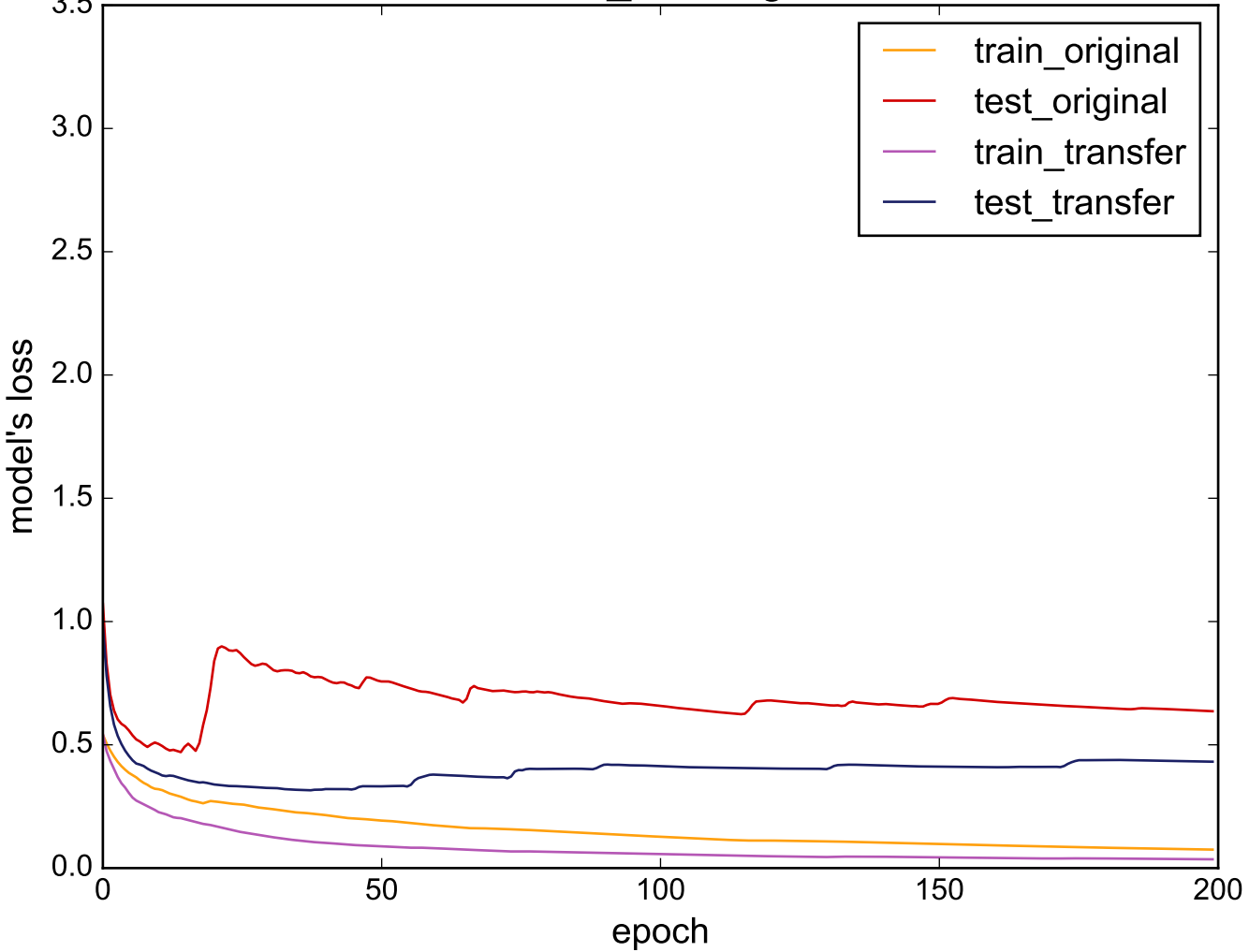
Source: Cricket_Z - Target: ECG200
