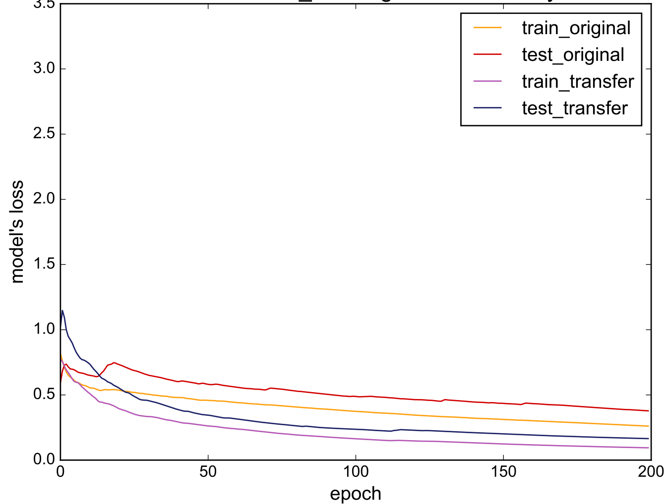
Source: Cricket_Z - Target: ECGFiveDays
