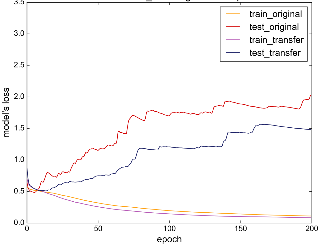
Source: Cricket_Z - Target: Earthquakes
