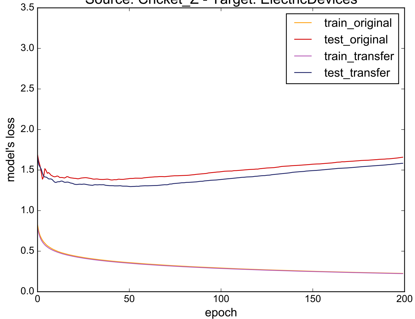
Source: Cricket_Z - Target: ElectricDevices
