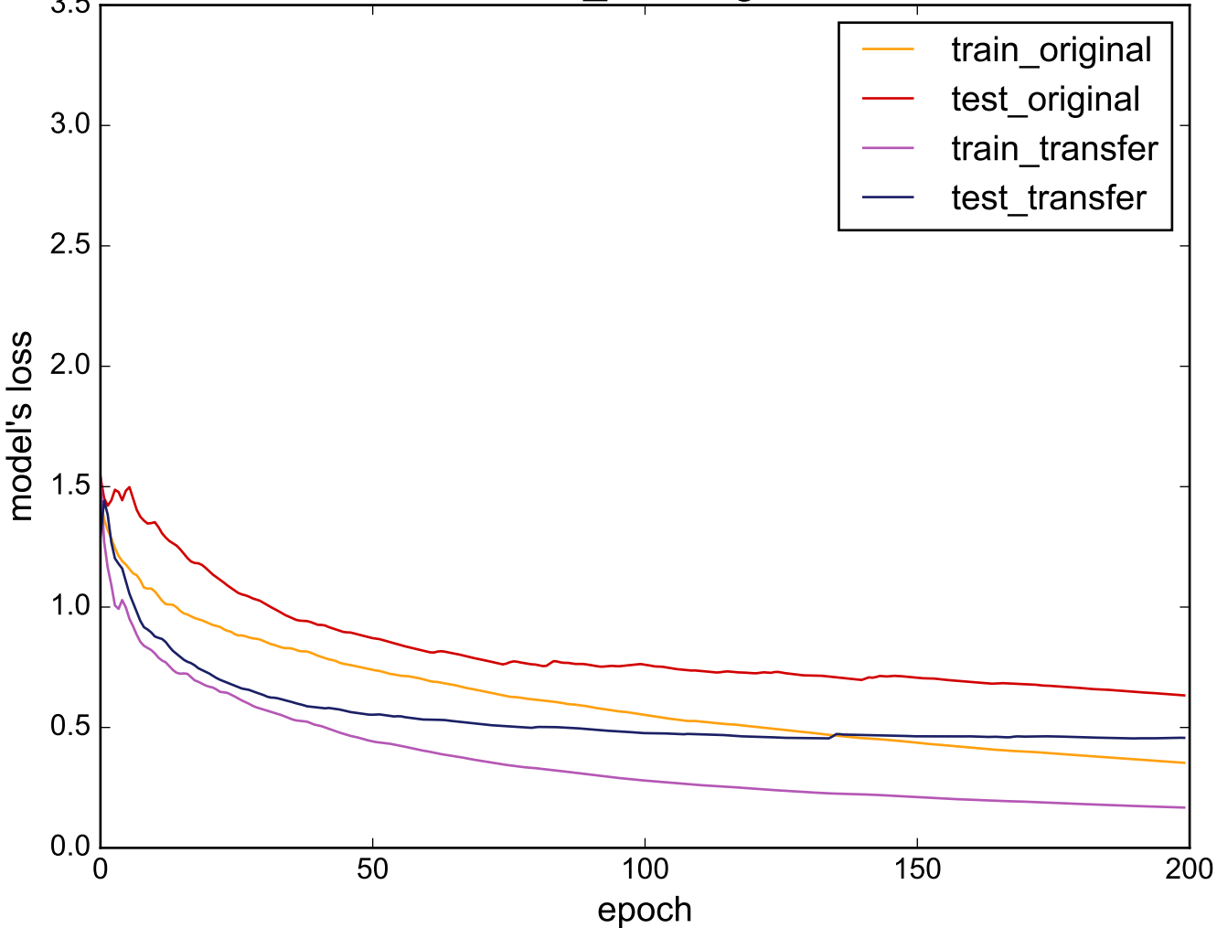
Source: Cricket_Z - Target: FaceFour
