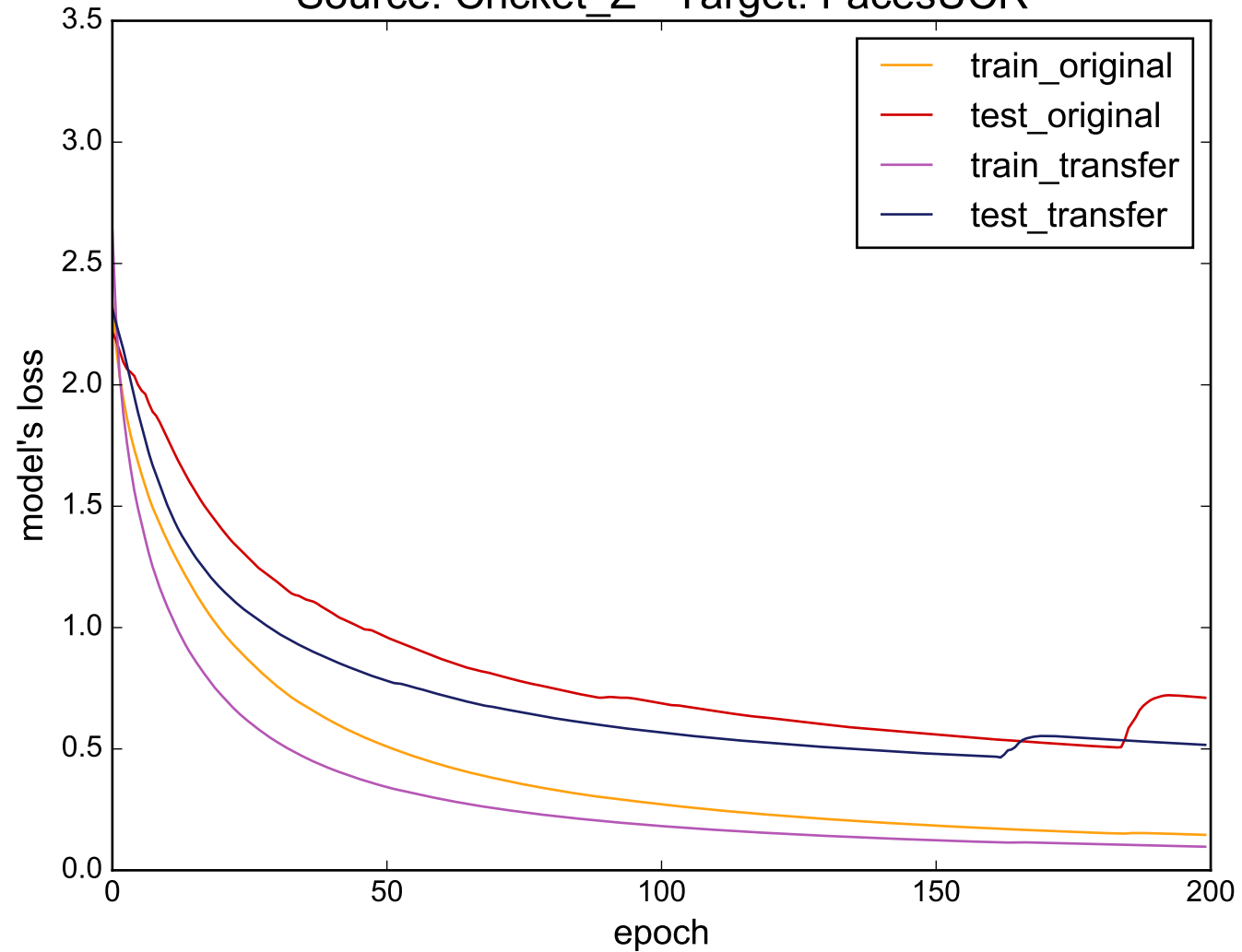
Source: Cricket_Z - Target: FacesUCR
