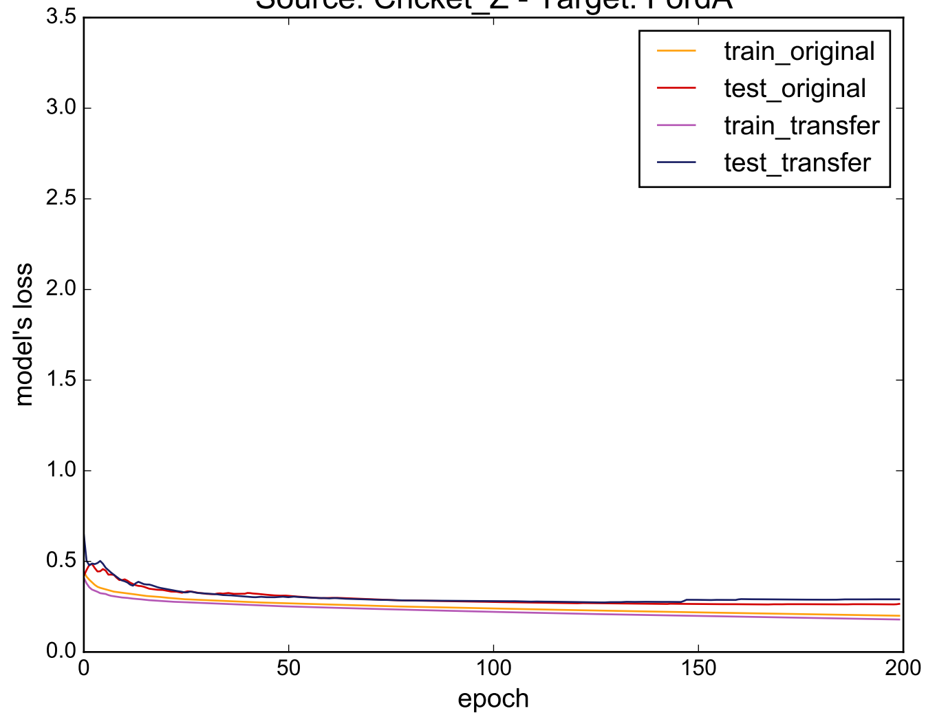
Source: Cricket_Z - Target: FordA
