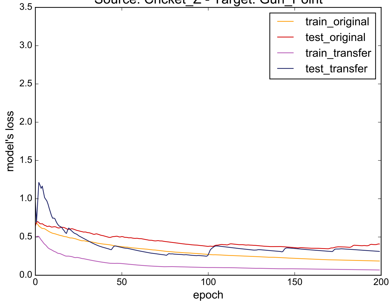
Source: Cricket_Z - Target: Gun_Point
