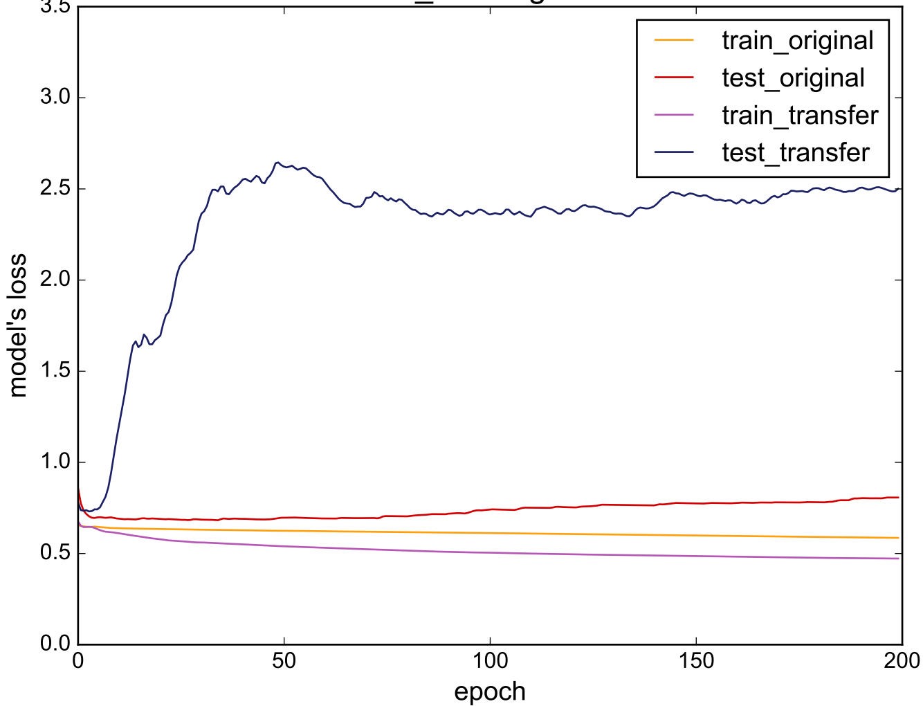
Source: Cricket_Z - Target: HandOutlines
