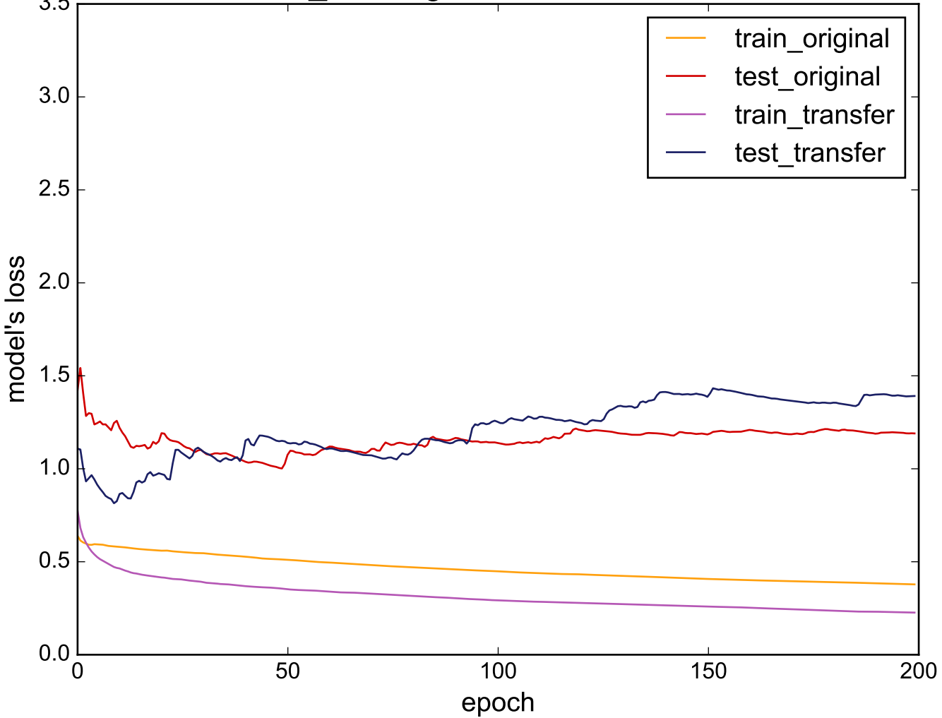
Source: Cricket_Z - Target: MiddlePhalanxOutlineCorrect
