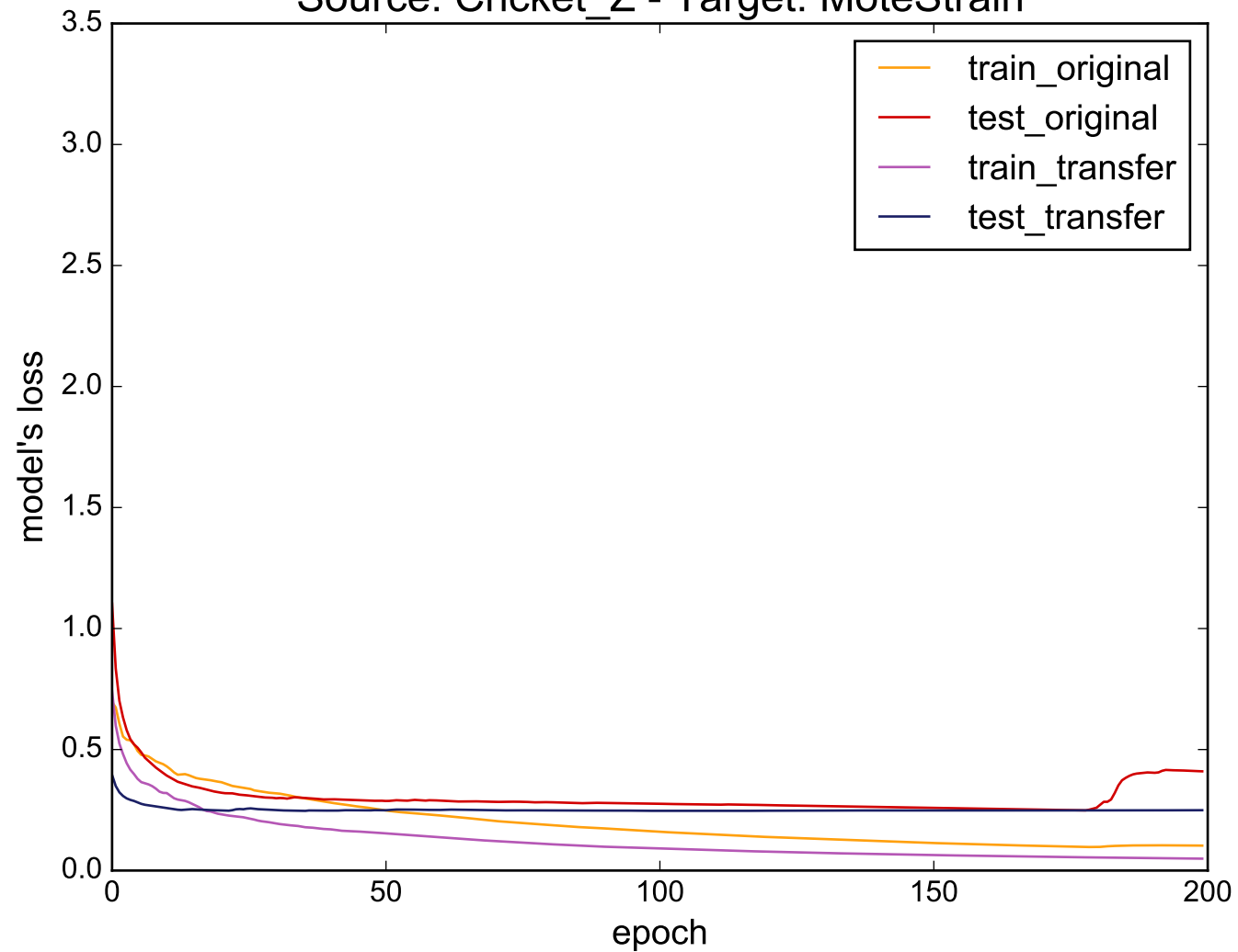
Source: Cricket_Z - Target: MoteStrain
