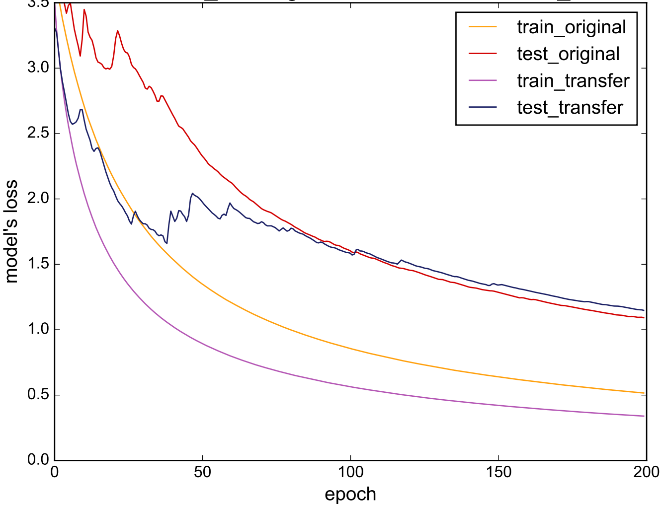
Source: Cricket_Z - Target: NonInvasiveFatalECG_Thorax1
