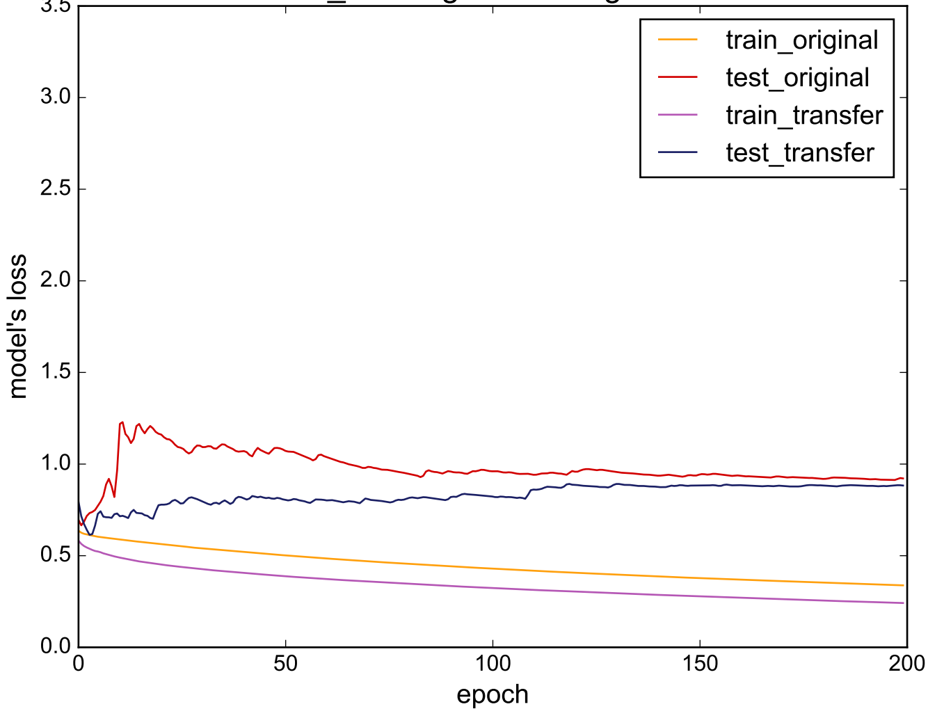
Source: Cricket_Z - Target: PhalangesOutlinesCorrect
