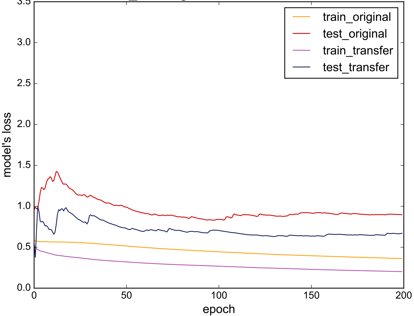
Source: Cricket_Z - Target: ProximalPhalanxOutlineCorrect
