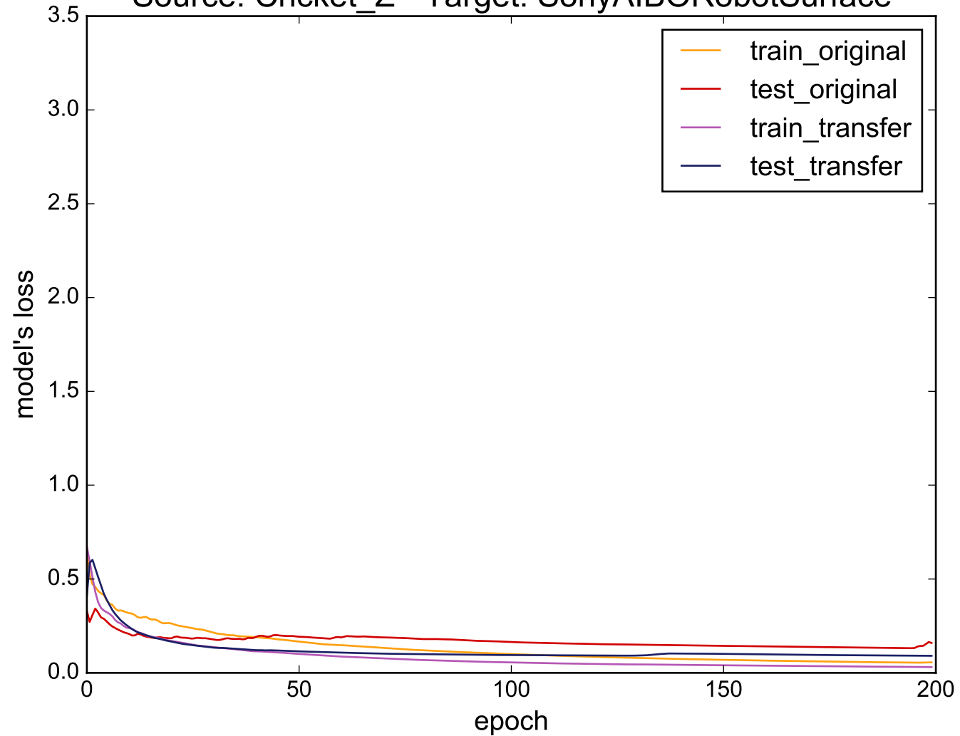
Source: Cricket_Z - Target: SonyAIBORobotSurface
