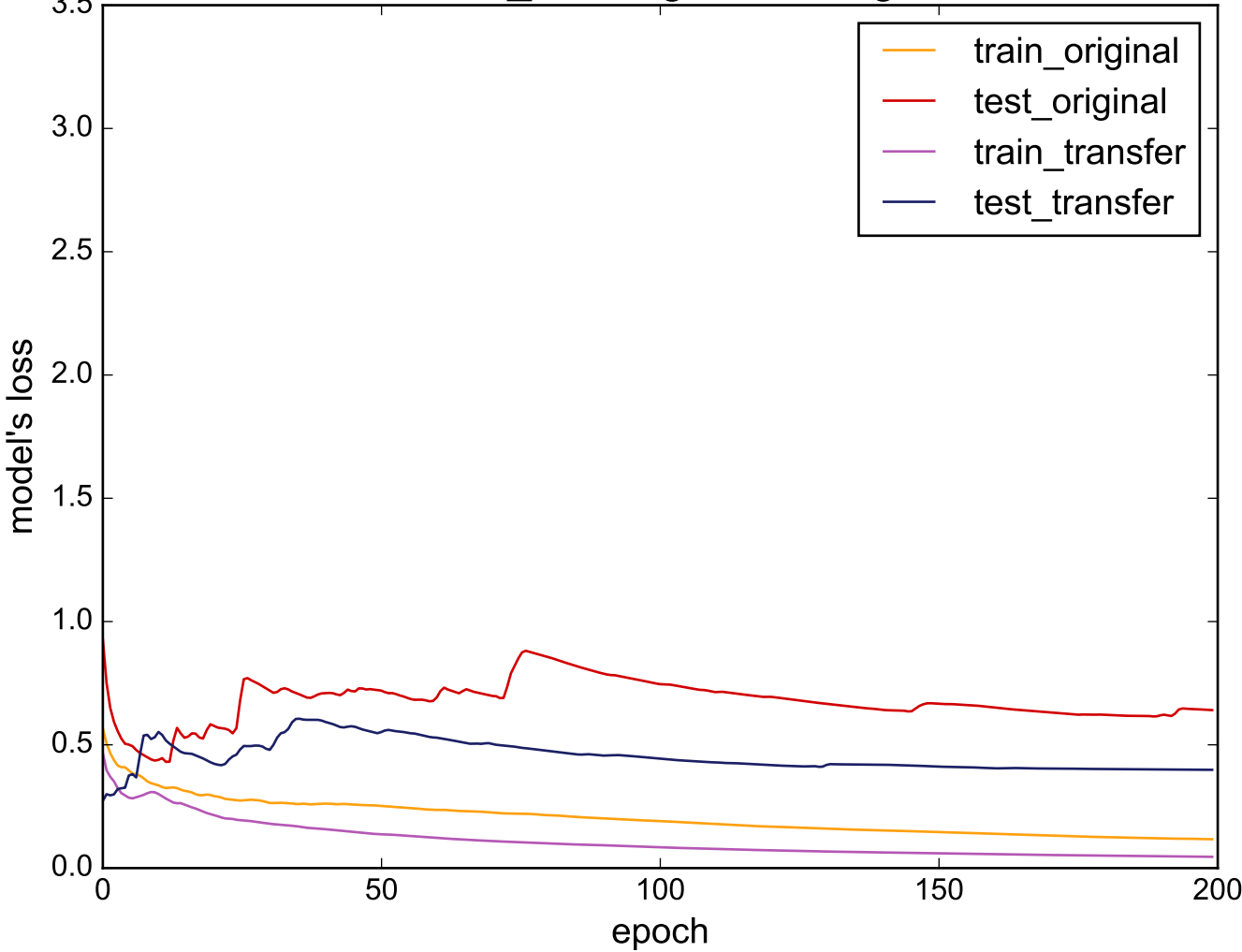
Source: Cricket_Z - Target: ToeSegmentation2
