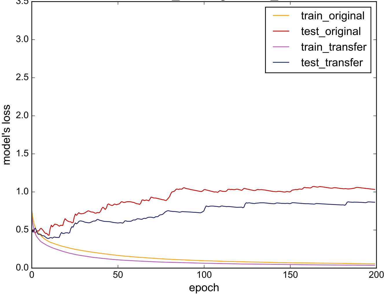
Source: Cricket_Z - Target: Two_Patterns
