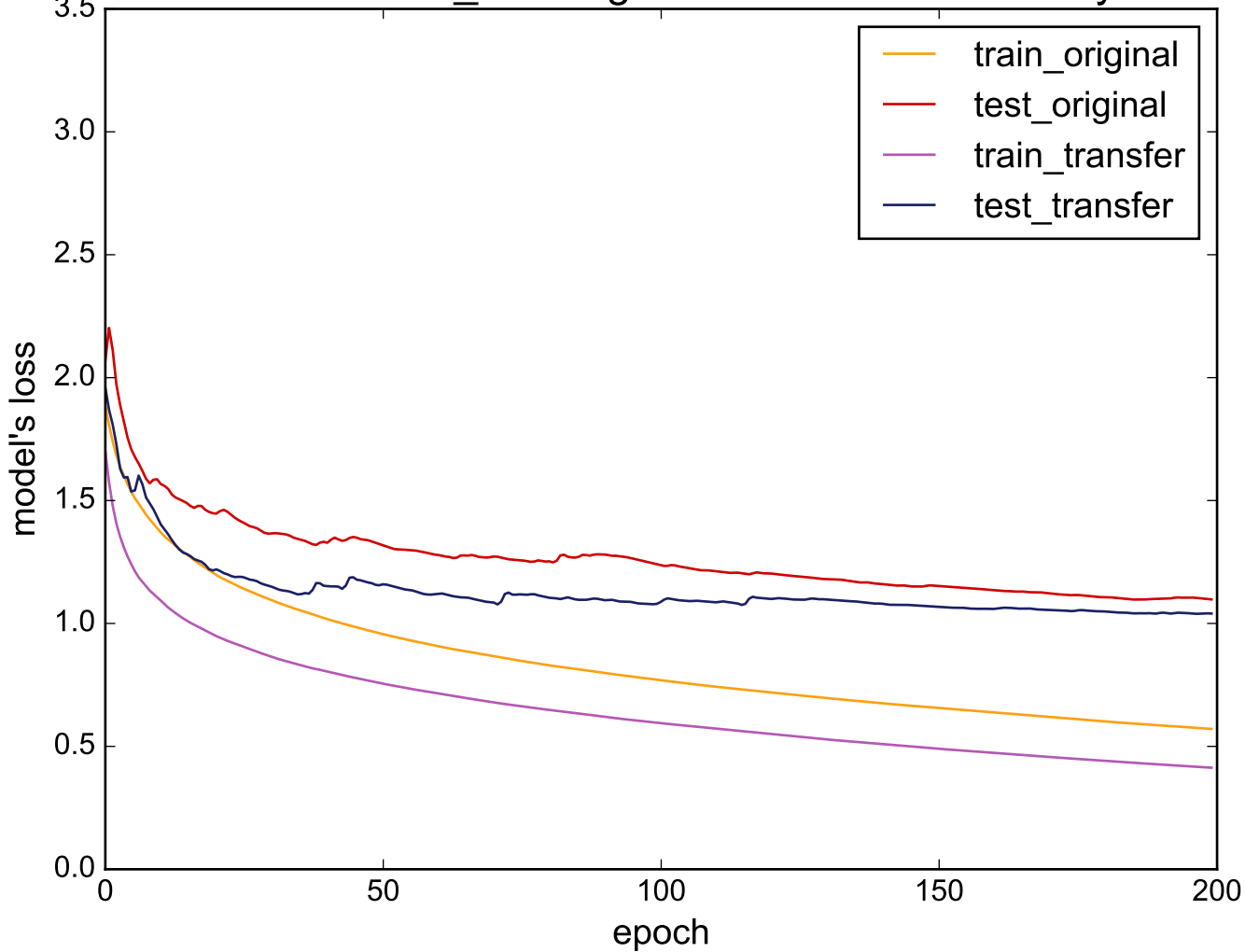
Source: Cricket_Z - Target: UWaveGestureLibraryAll
