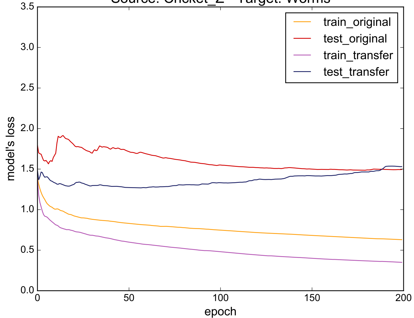
Source: Cricket_Z - Target: Worms
