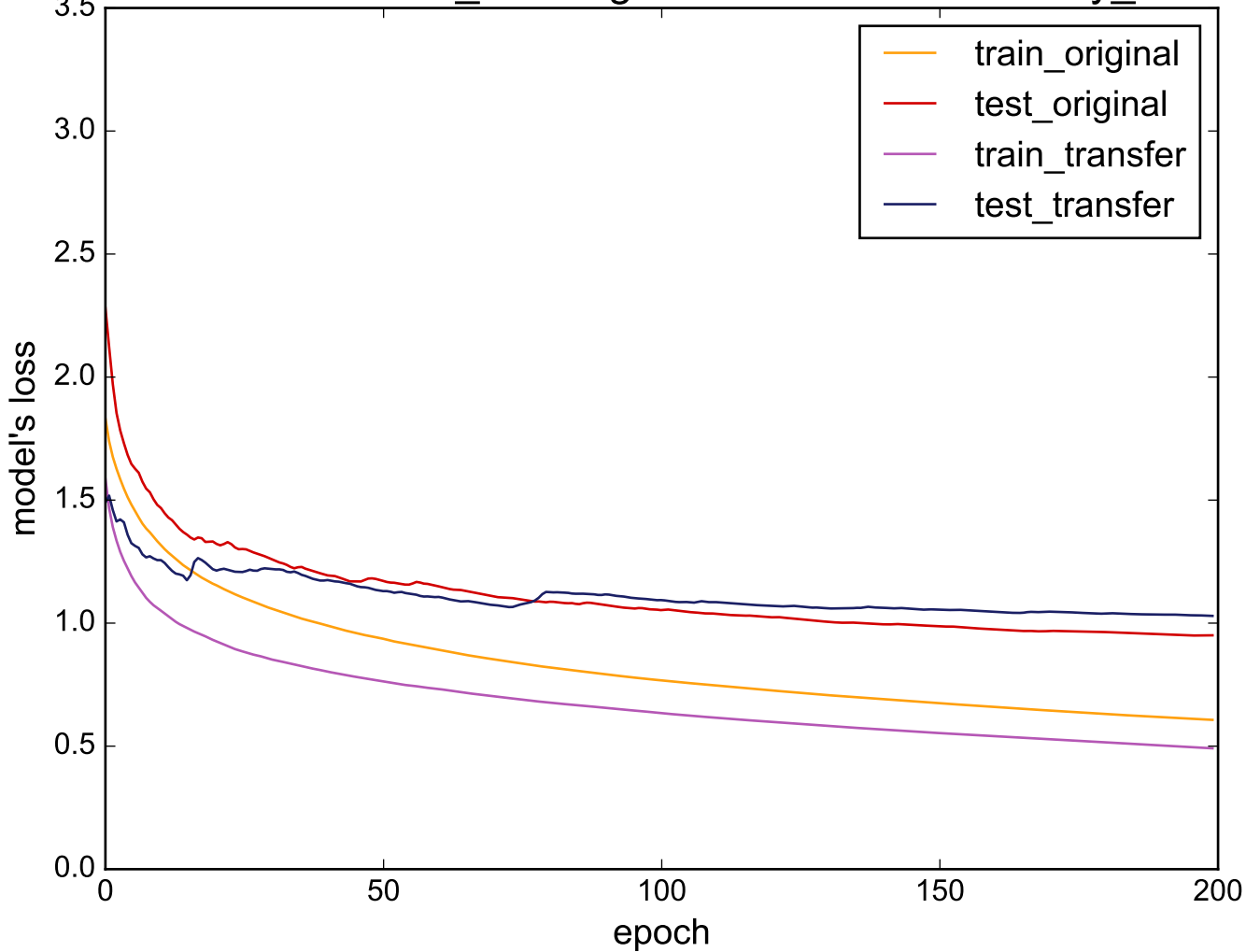
Source: Cricket_Z - Target: uWaveGestureLibrary_X
