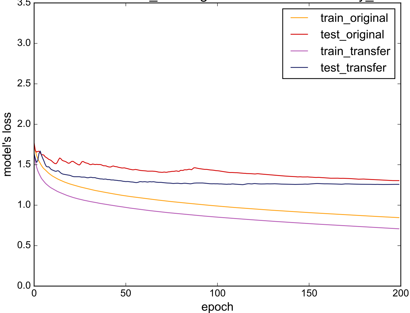
Source: Cricket_Z - Target: uWaveGestureLibrary_Y
