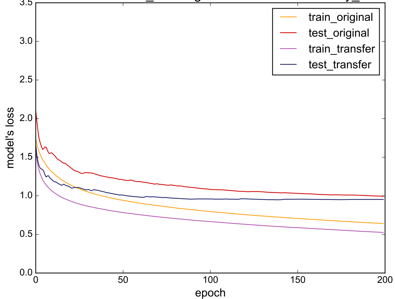
Source: Cricket_Z - Target: uWaveGestureLibrary_Z
