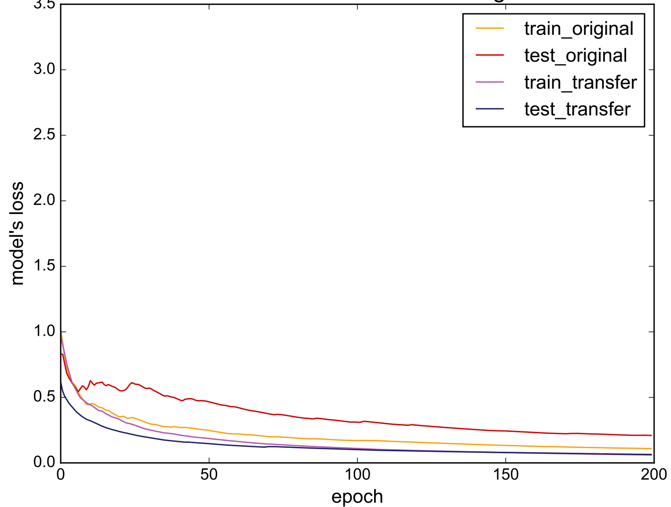
Source: DiatomSizeReduction - Target: CBF
