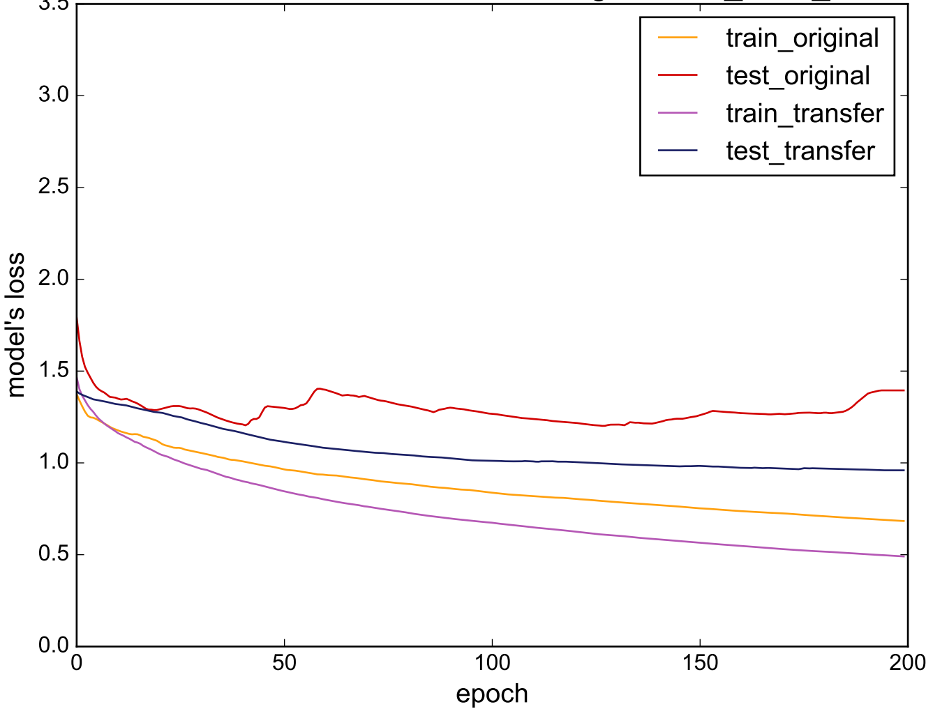
Source: DiatomSizeReduction - Target: CinC_ECG_torso
