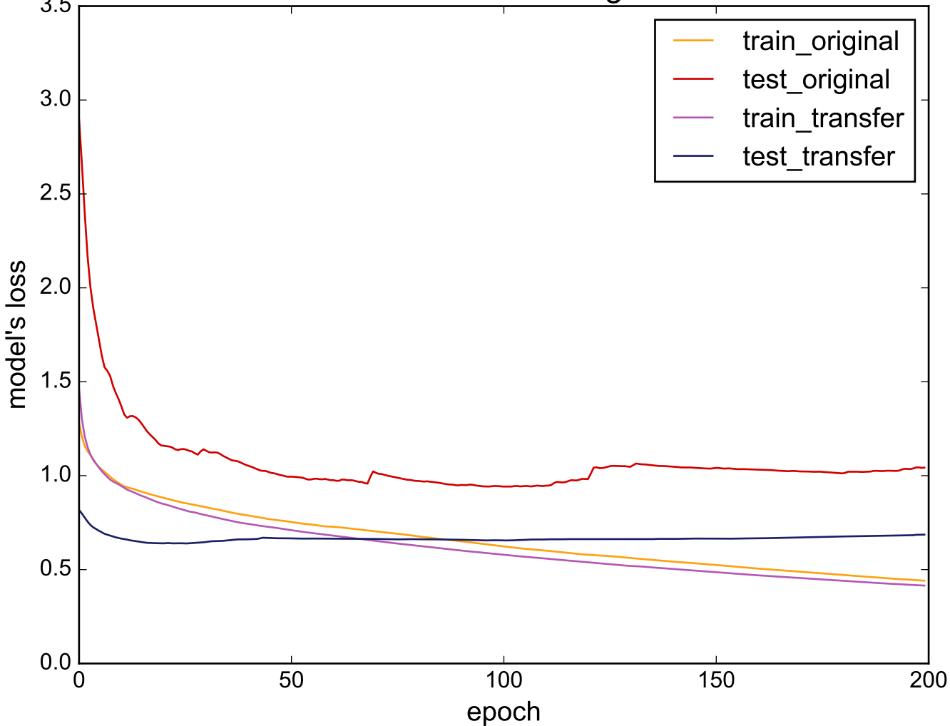
Source: DiatomSizeReduction - Target: DistalPhalanxTW
