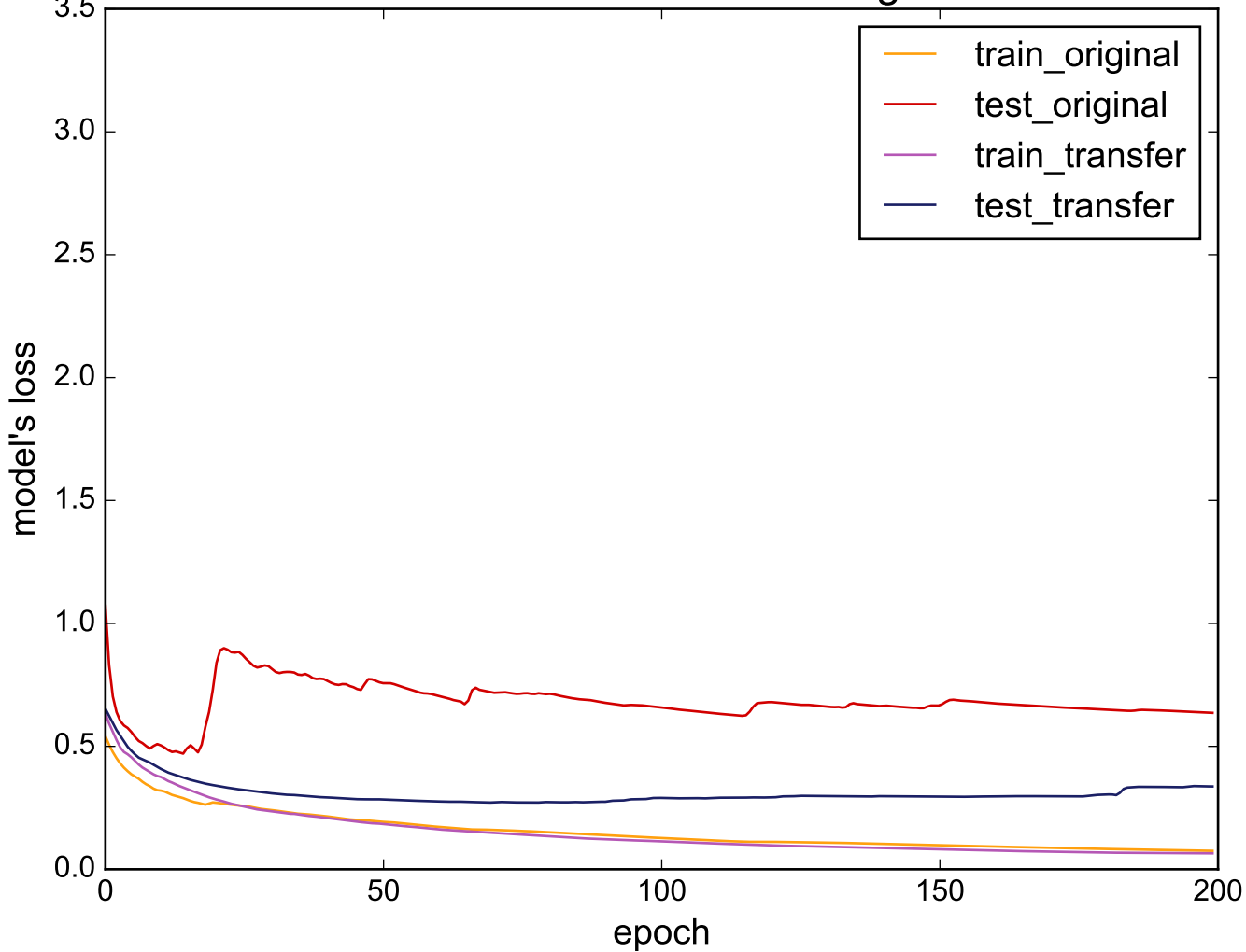
Source: DiatomSizeReduction - Target: ECG200
