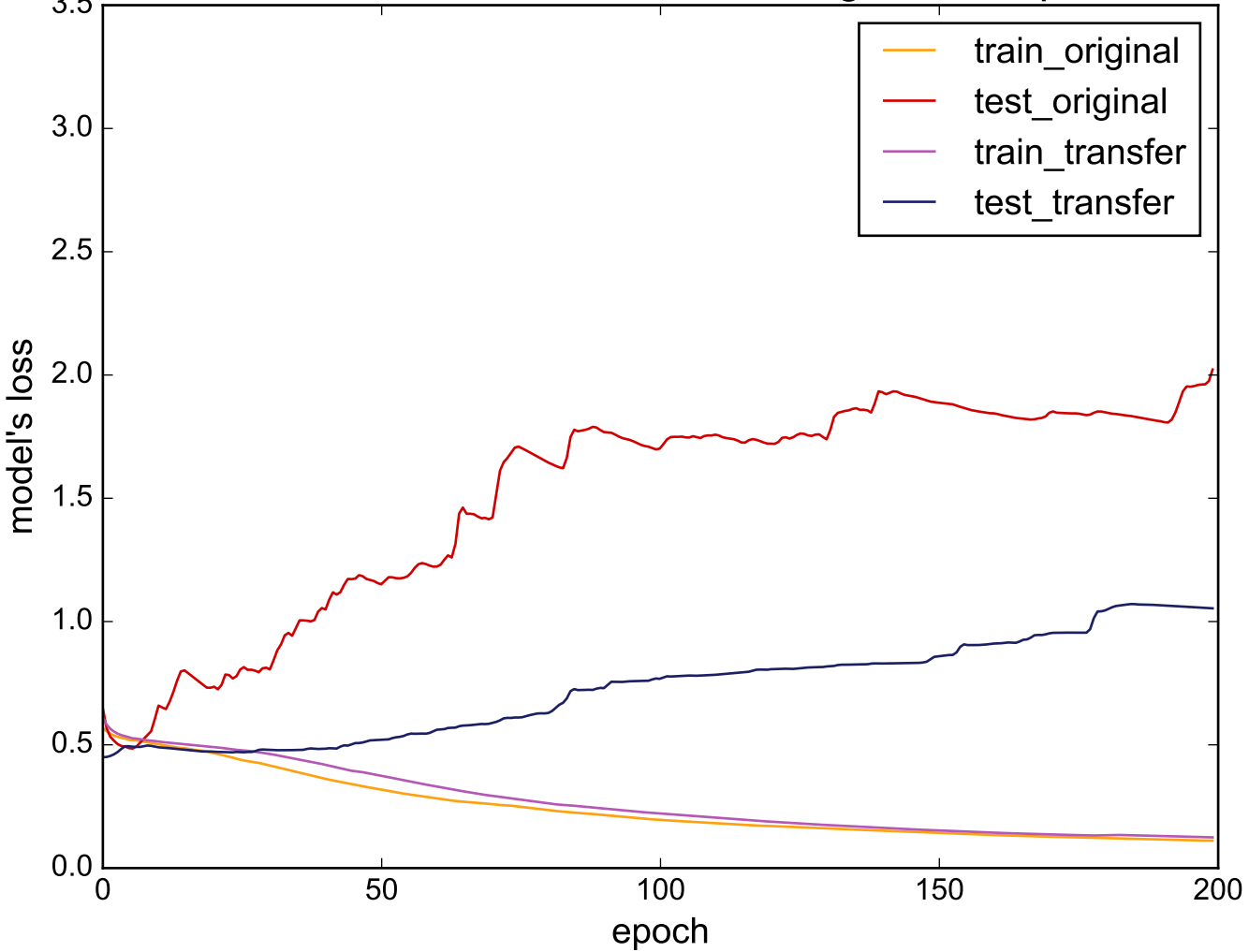
Source: DiatomSizeReduction - Target: Earthquakes
