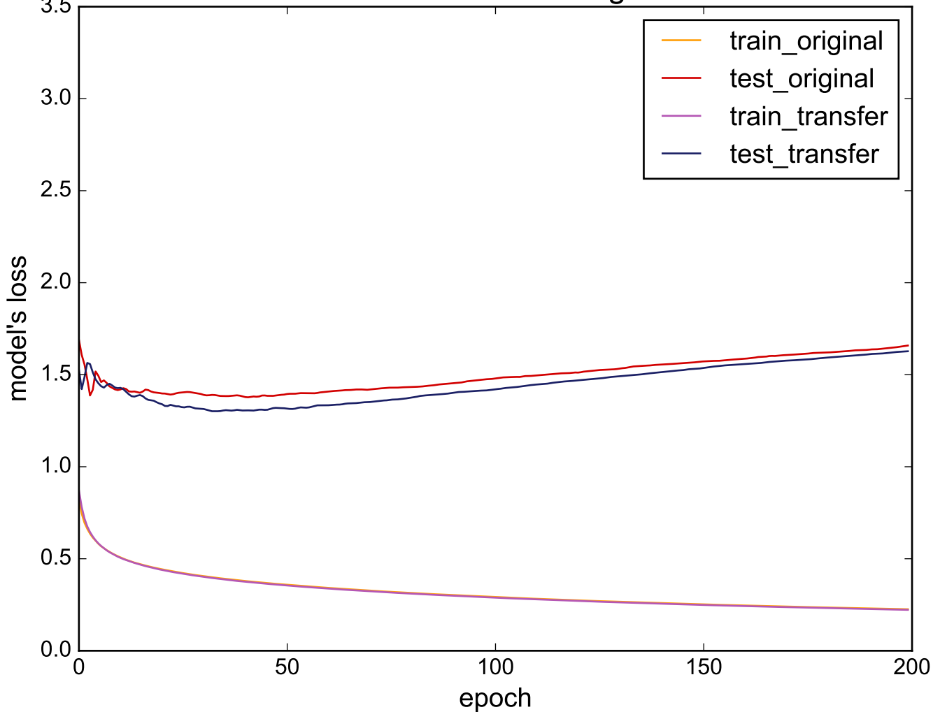
Source: DiatomSizeReduction - Target: ElectricDevices
