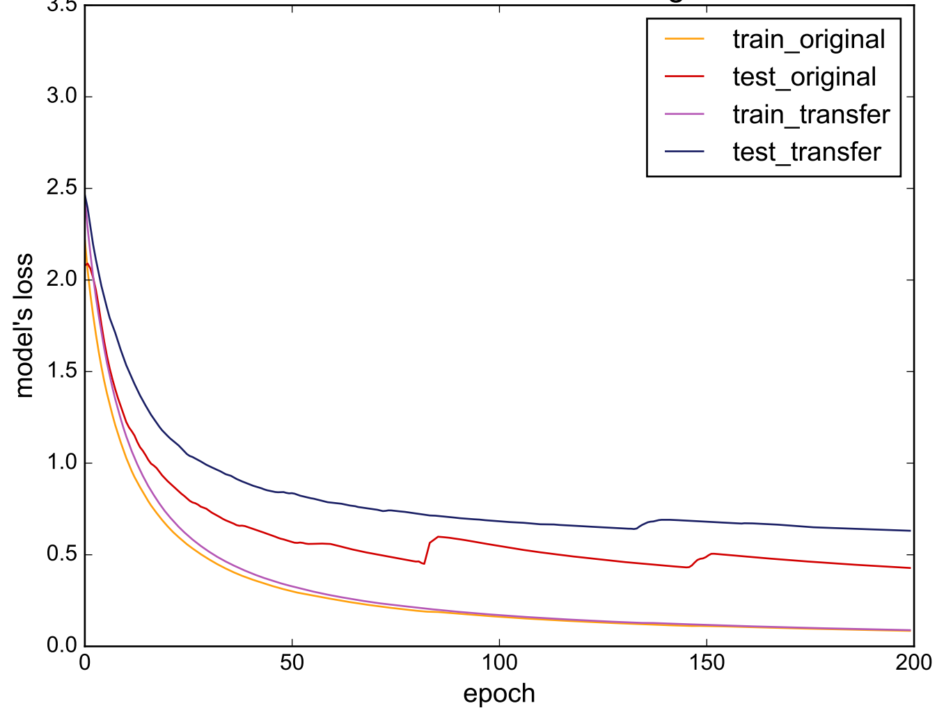
Source: DiatomSizeReduction - Target: FaceAll
