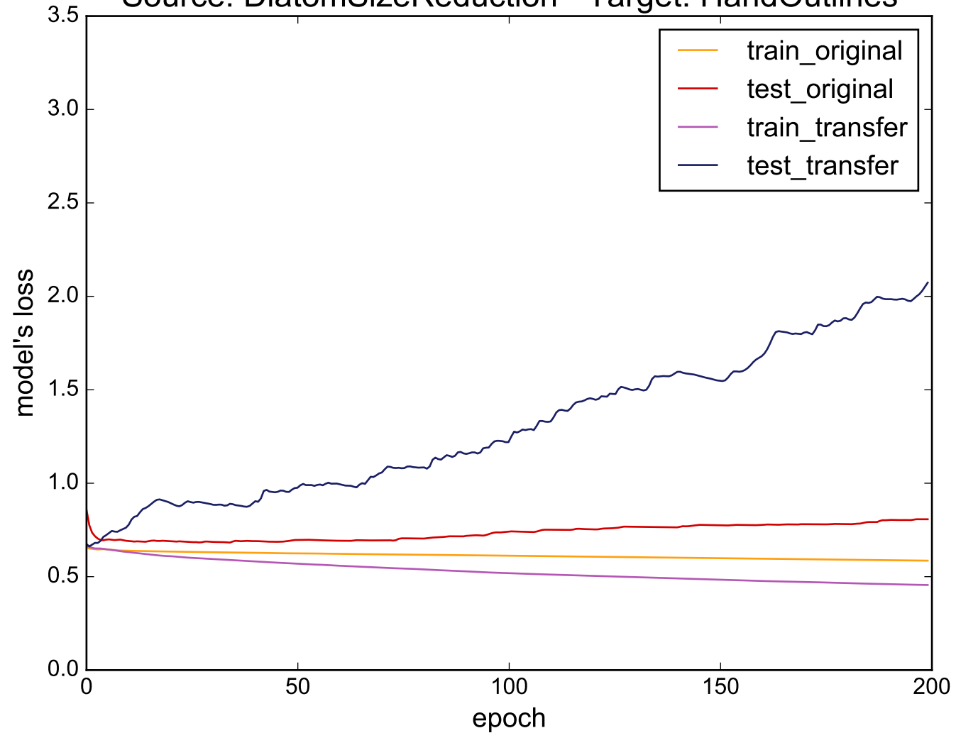
Source: DiatomSizeReduction - Target: HandOutlines
