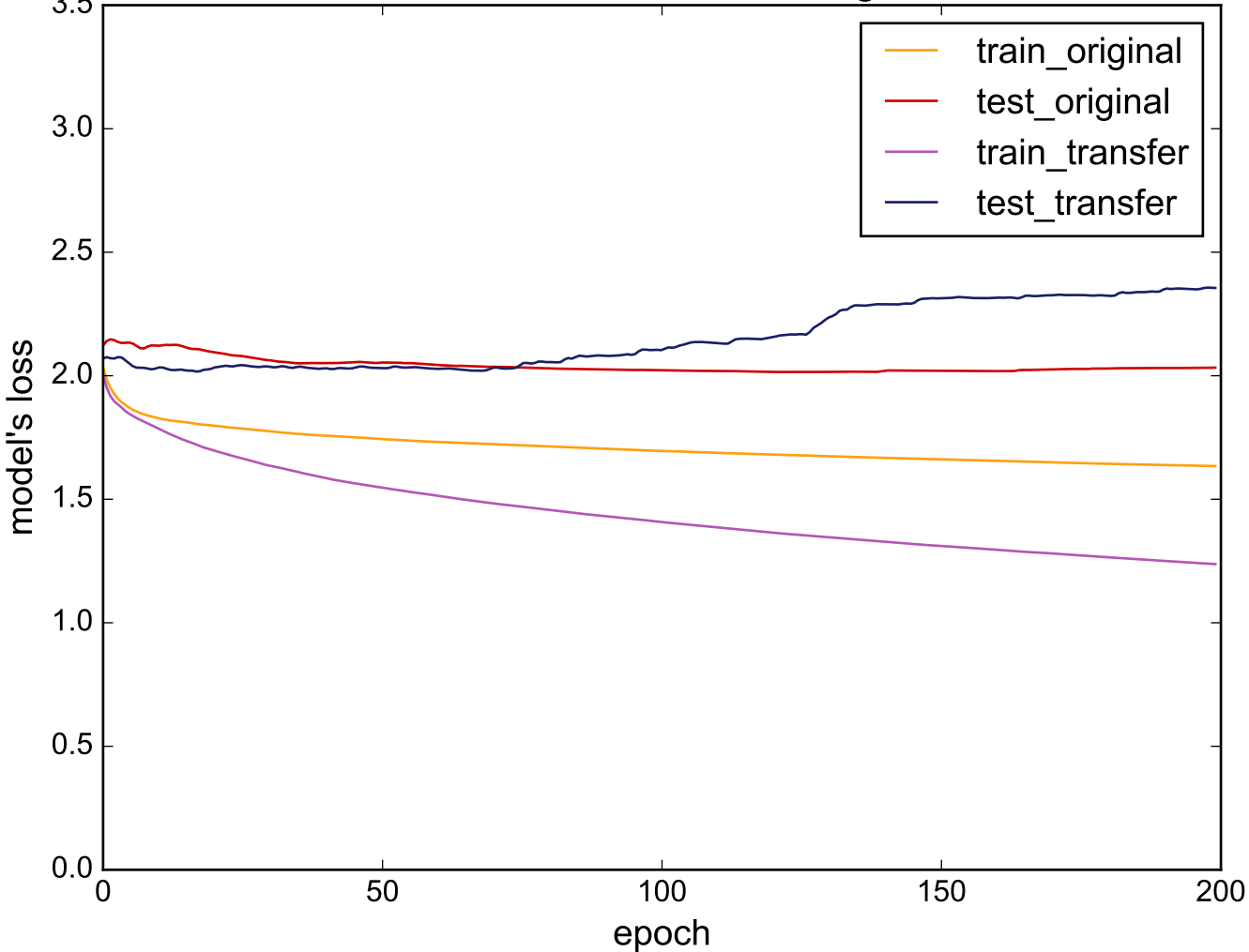
Source: DiatomSizeReduction - Target: InlineSkate
