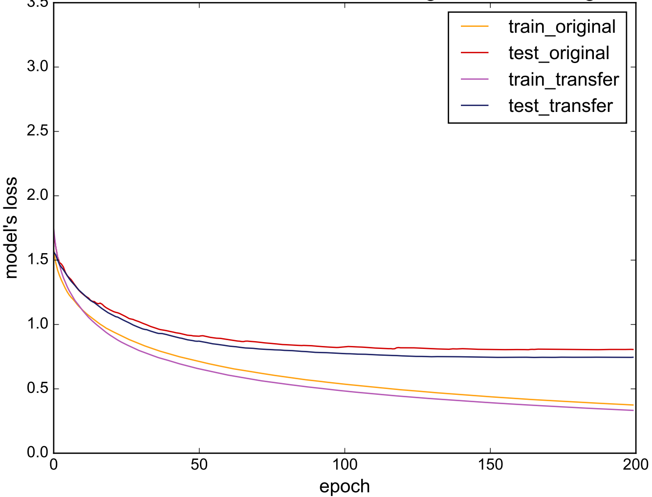
Source: DiatomSizeReduction - Target: MedicalImages
