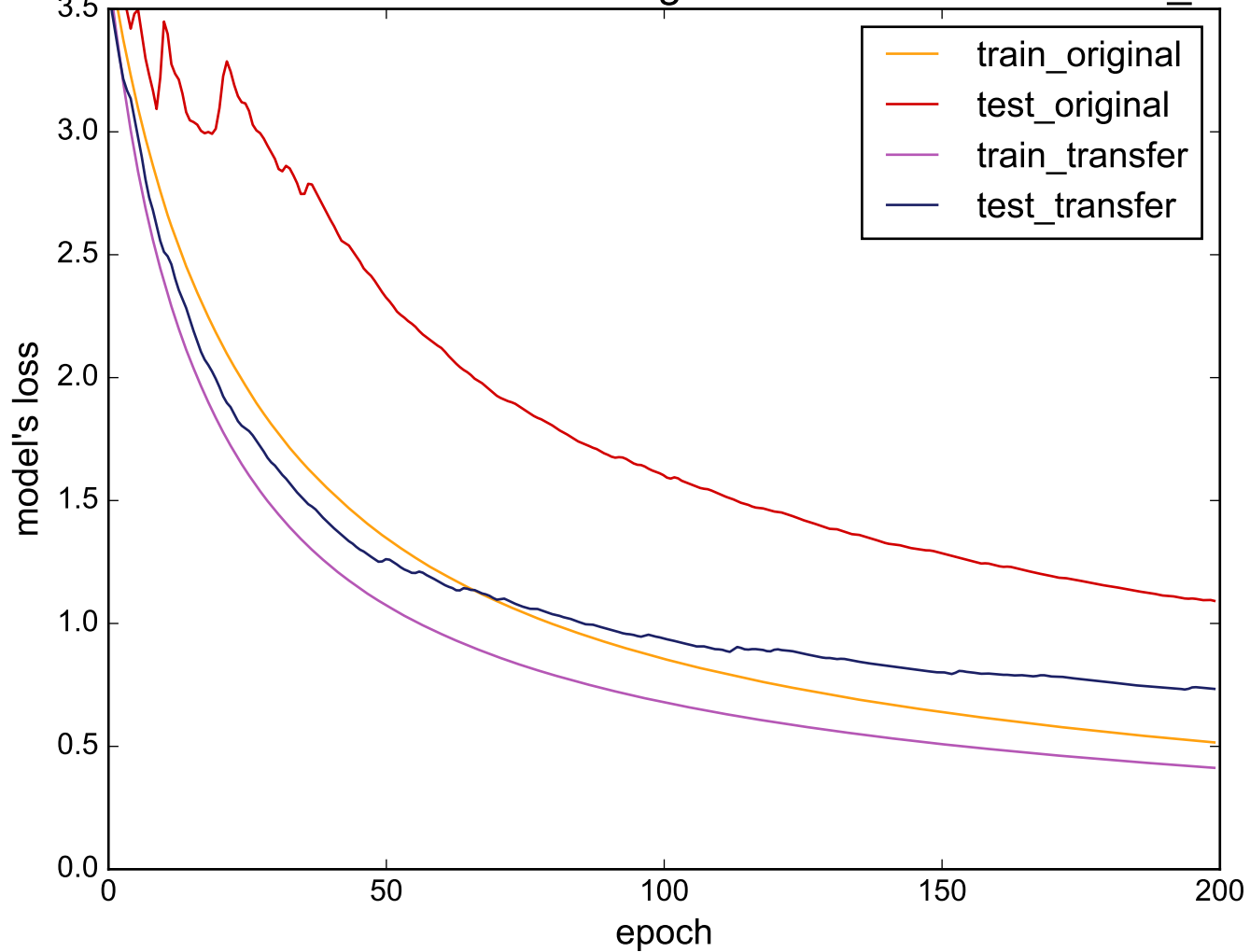
Source: DiatomSizeReduction - Target: NonInvasiveFatalECG_Thorax1
