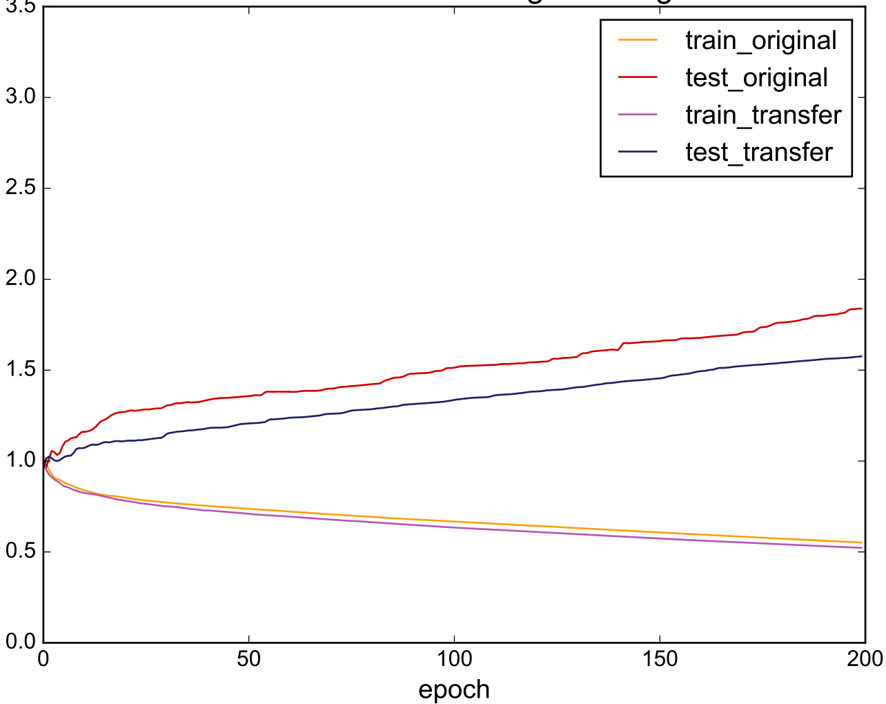
Source: DiatomSizeReduction - Target: RefrigerationDevices
