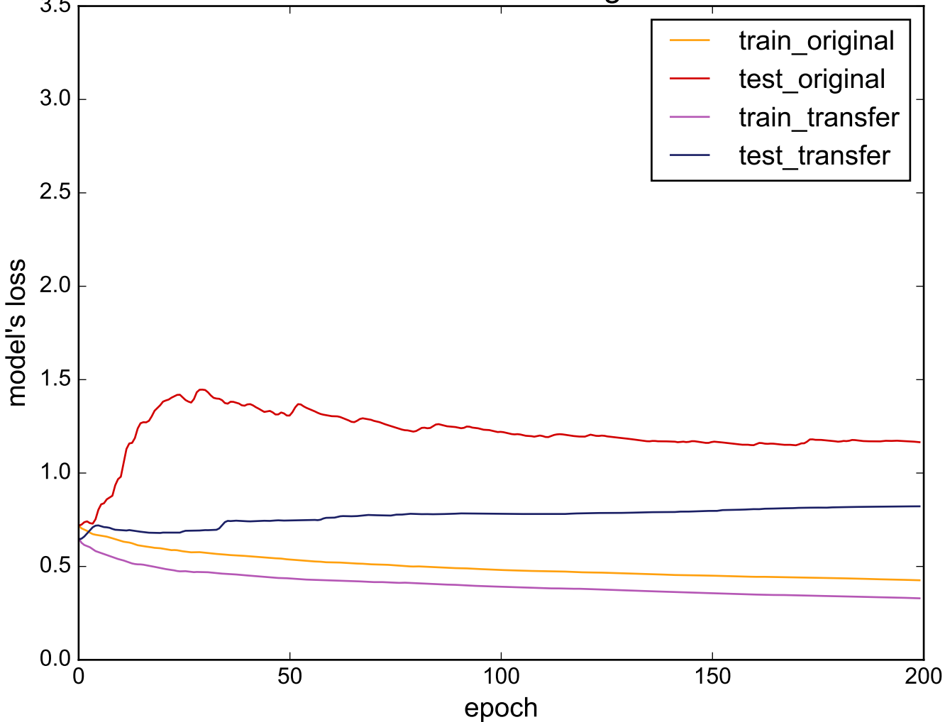
Source: DiatomSizeReduction - Target: WormsTwoClass
