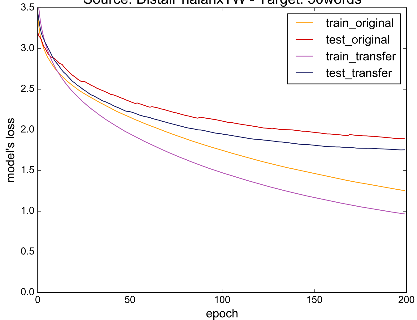
Source: DistalPhalanxTW - Target: 50words
