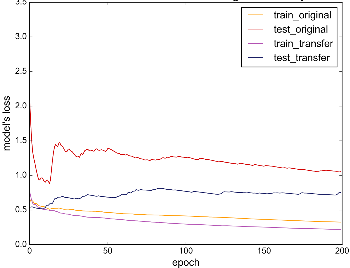
Source: DistalPhalanxTW - Target: BeetleFly
