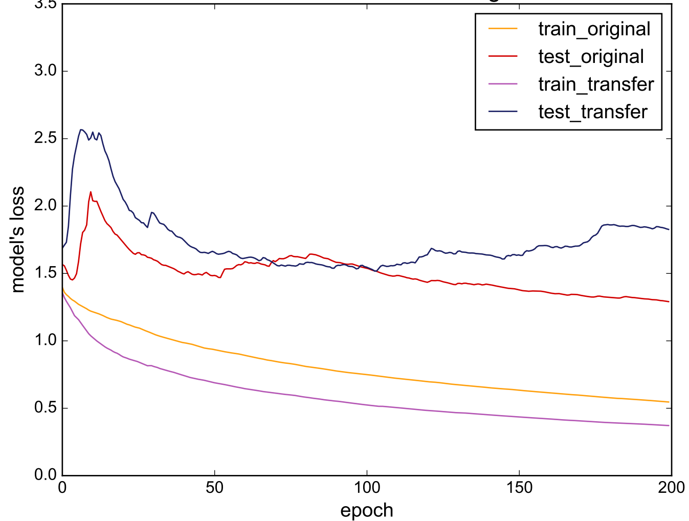
Source: DistalPhalanxTW - Target: Car
