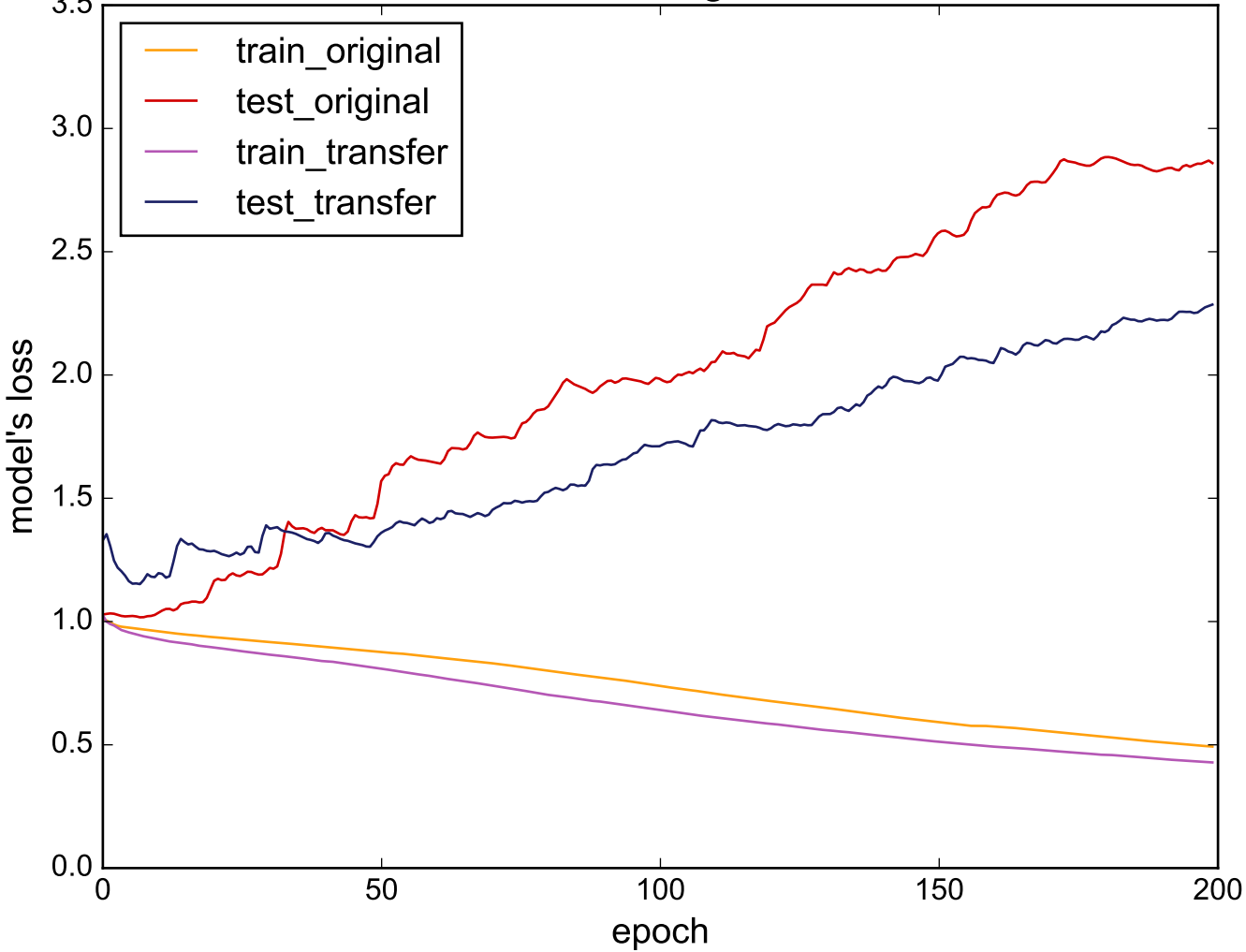
Source: DistalPhalanxTW - Target: ChlorineConcentration
