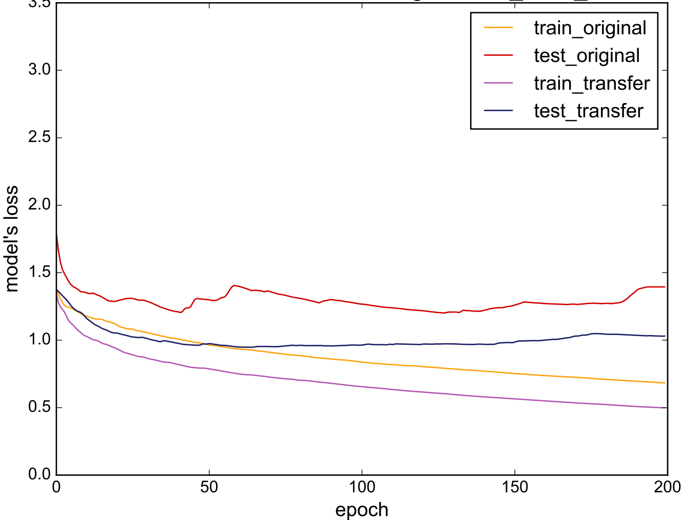
Source: DistalPhalanxTW - Target: CinC_ECG_torso
