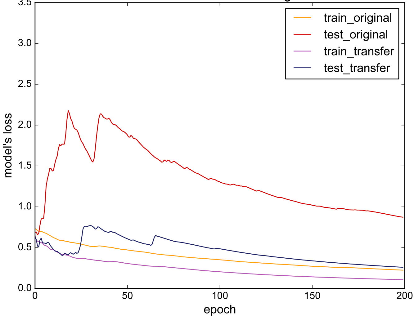
Source: DistalPhalanxTW - Target: Coffee
