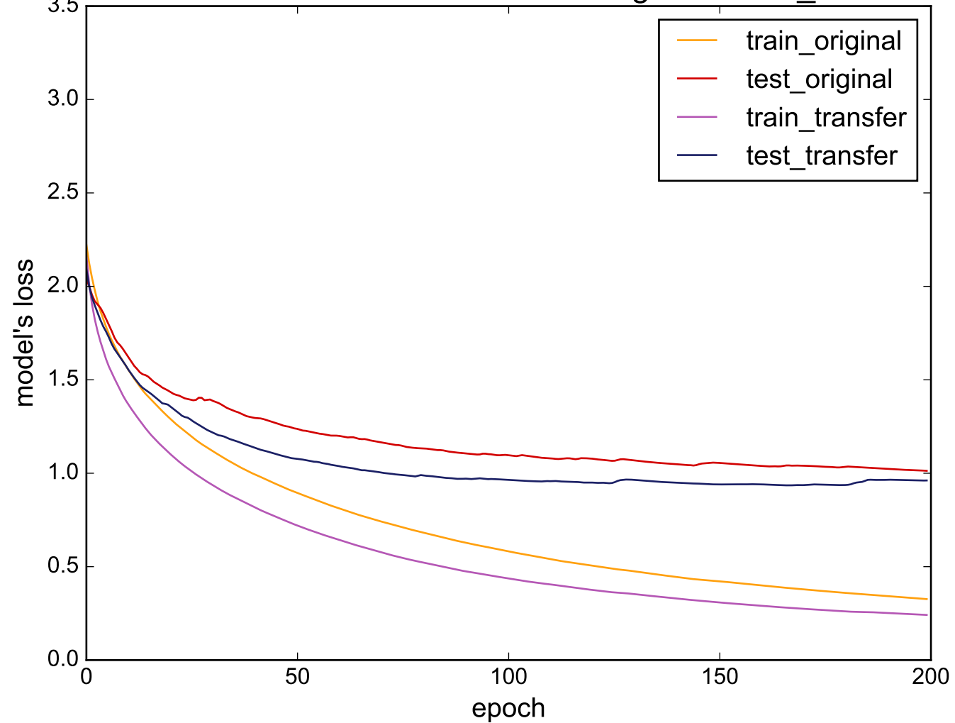
Source: DistalPhalanxTW - Target: Cricket_X
