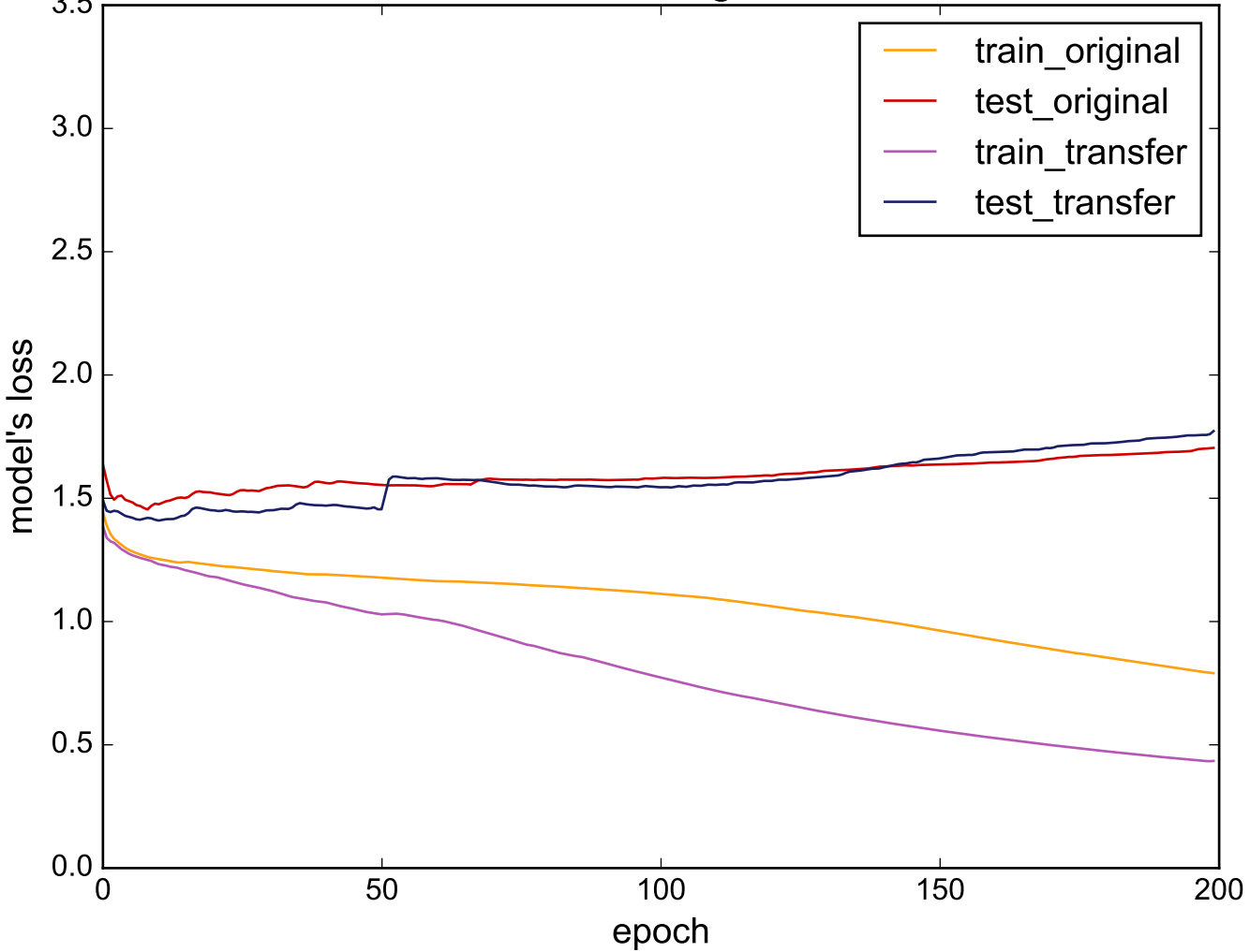
Source: DistalPhalanxTW - Target: DiatomSizeReduction
